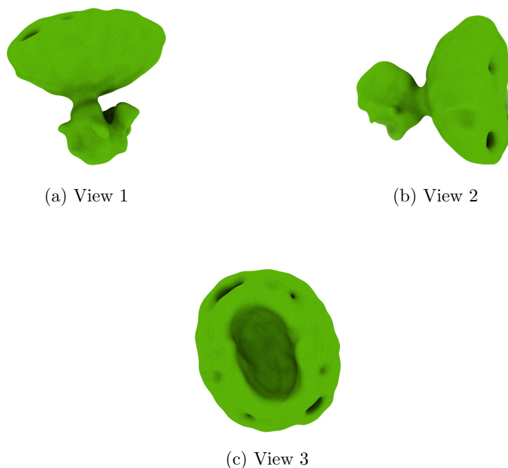
Figure 4: Isosurface at threshold=0.016900. Views generated by ChimeraX at a the following X, Y, Z angles: View 1 (0, -90, -90), View 2 (-90, 0, -90), View 3 (0, 0, 0).
