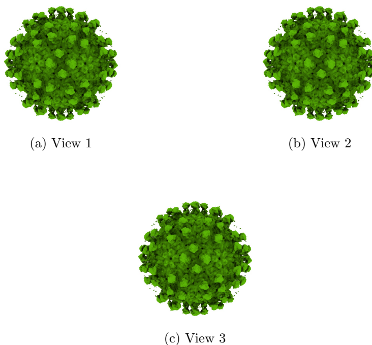
Figure 4: Isosurface at threshold=0.036500. Views generated by ChimeraX at a the following X, Y, Z angles: View 1 (0, -90, -90), View 2 (-90, 0, -90), View 3 (0, 0, 0).
