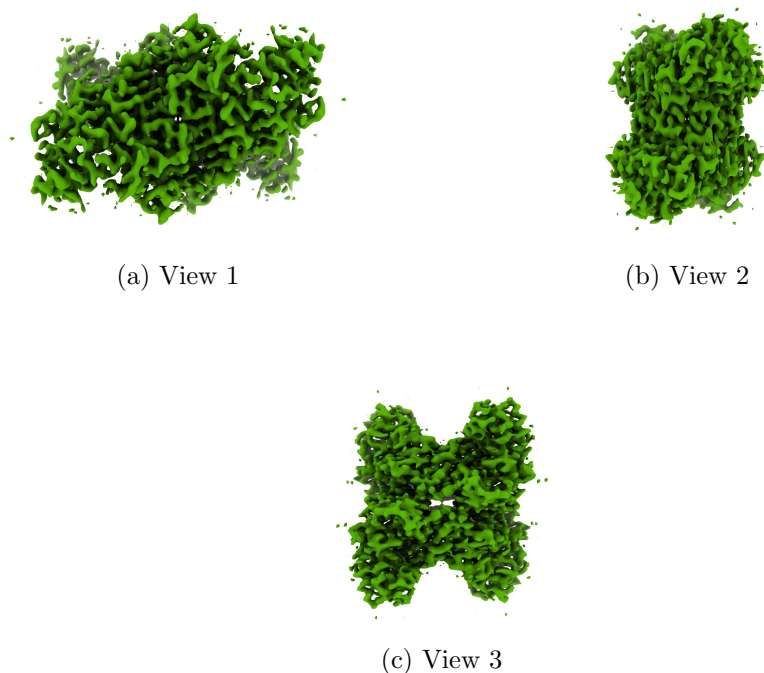
Figure 4: Isosurface at threshold=0.383000. Views generated by ChimeraX at a the following X, Y, Z angles: View 1 (0, -90, -90), View 2 (-90, 0, -90), View 3 (0, 0, 0).
