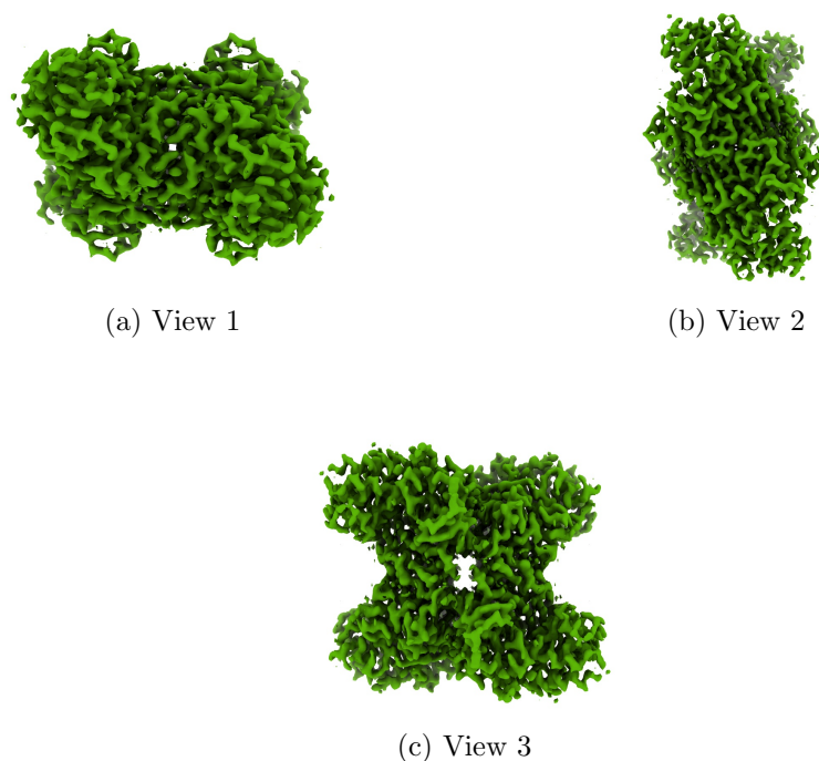
Figure 4: Isosurface at threshold=0.644000. Views generated by ChimeraX at a the following X, Y, Z angles: View 1 (0, -90, -90), View 2 (-90, 0, -90), View 3 (0, 0, 0).
