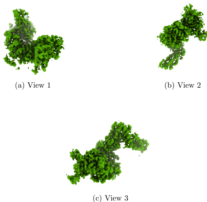
Figure 4: Isosurface at threshold=0.600000. Views generated by ChimeraX at a the following X, Y, Z angles: View 1 (0, -90, -90), View 2 (-90, 0, -90), View 3 (0, 0, 0).
