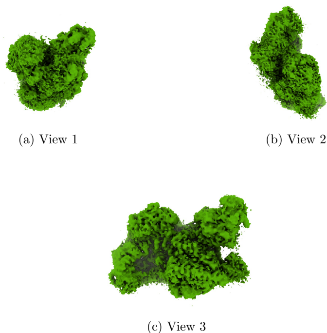
Figure 4: Isosurface at threshold=0.024800. Views generated by ChimeraX at a the following X, Y, Z angles: View 1 (0, -90, -90), View 2 (-90, 0, -90), View 3 (0, 0, 0).
