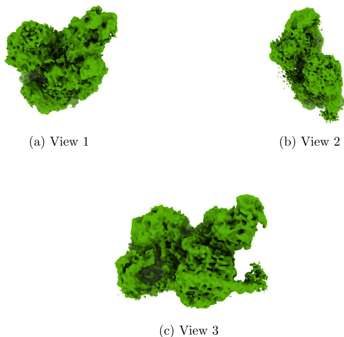
Figure 4: Isosurface at threshold=0.028500. Views generated by ChimeraX at a the following X, Y, Z angles: View 1 (0, -90, -90), View 2 (-90, 0, -90), View 3 (0, 0, 0).
