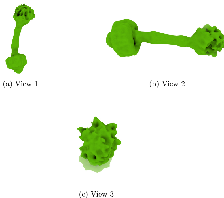
Figure 4: Isosurface at threshold=0.261000. Views generated by ChimeraX at a the following X, Y, Z angles: View 1 (0, -90, -90), View 2 (-90, 0, -90), View 3 (0, 0, 0).
