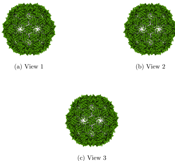
Figure 4: Isosurface at threshold=0.070600. Views generated by ChimeraX at a the following X, Y, Z angles: View 1 (0, -90, -90), View 2 (-90, 0, -90), View 3 (0, 0, 0).
