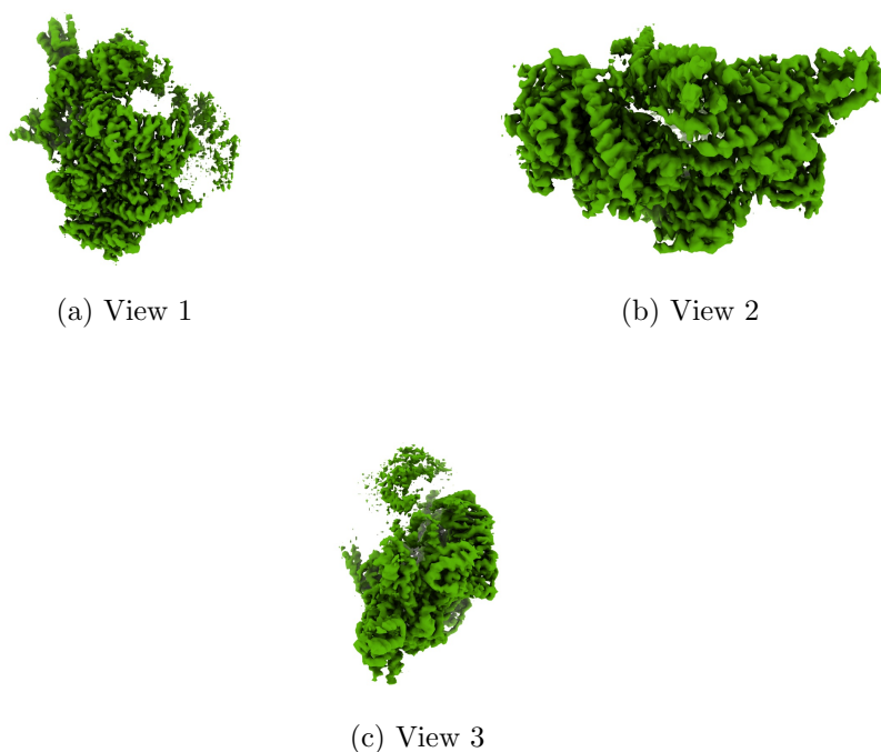
Figure 4: Isosurface at threshold=0.038900. Views generated by ChimeraX at a the following X, Y, Z angles: View 1 (0, -90, -90), View 2 (-90, 0, -90), View 3 (0, 0, 0).
