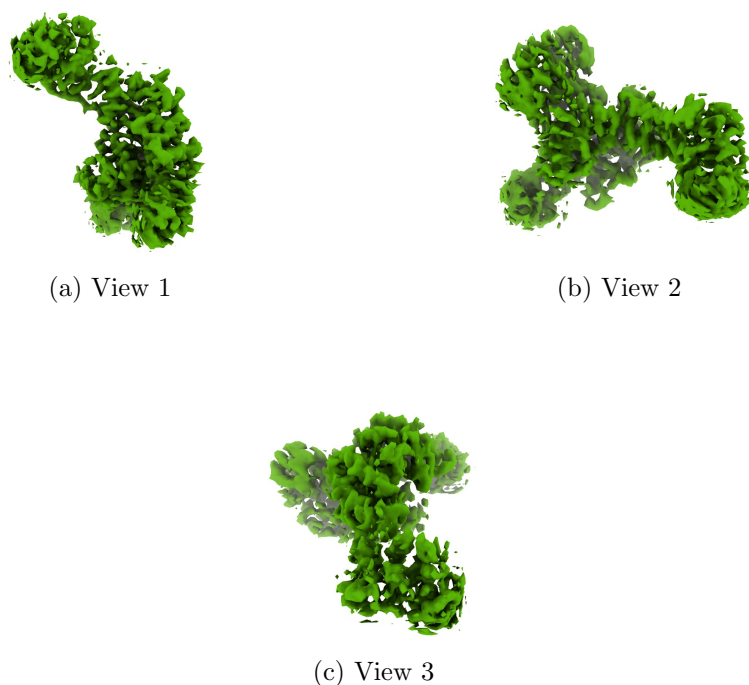
Figure 4: Isosurface at threshold=0.053500. Views generated by ChimeraX at a the following X, Y, Z angles: View 1 (0, -90, -90), View 2 (-90, 0, -90), View 3 (0, 0, 0).
