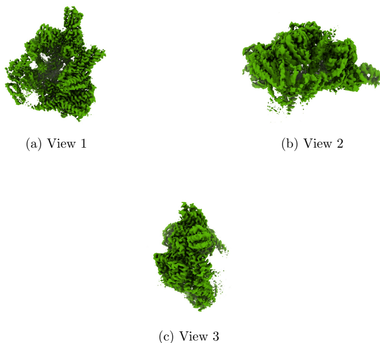
Figure 4: Isosurface at threshold=0.058100. Views generated by ChimeraX at a the following X, Y, Z angles: View 1 (0, -90, -90), View 2 (-90, 0, -90), View 3 (0, 0, 0).
