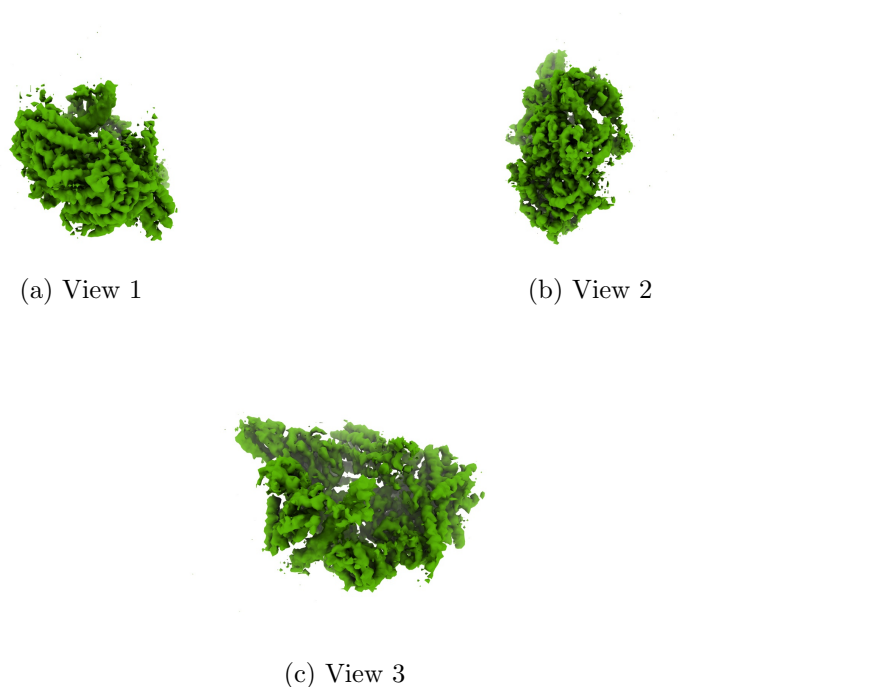
Figure 4: Isosurface at threshold=0.002450. Views generated by ChimeraX at a the following X, Y, Z angles: View 1 (0, -90, -90), View 2 (-90, 0, -90), View 3 (0, 0, 0).
