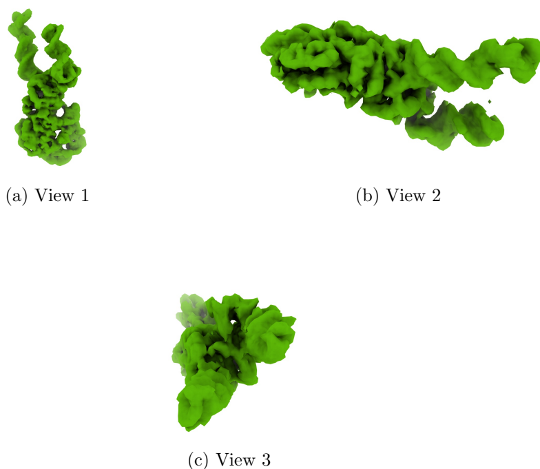
Figure 4: Isosurface at threshold=0.004600. Views generated by ChimeraX at a the following X, Y, Z angles: View 1 (0, -90, -90), View 2 (-90, 0, -90), View 3 (0, 0, 0).
