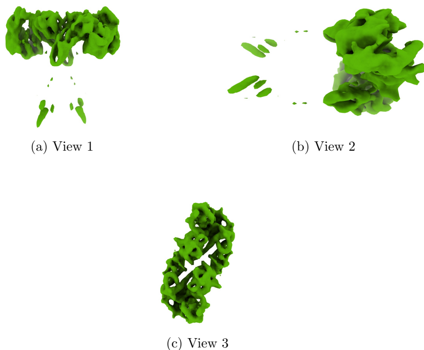
Figure 4: Isosurface at threshold=0.523000. Views generated by ChimeraX at a the following X, Y, Z angles: View 1 (0, -90, -90), View 2 (-90, 0, -90), View 3 (0, 0, 0).
