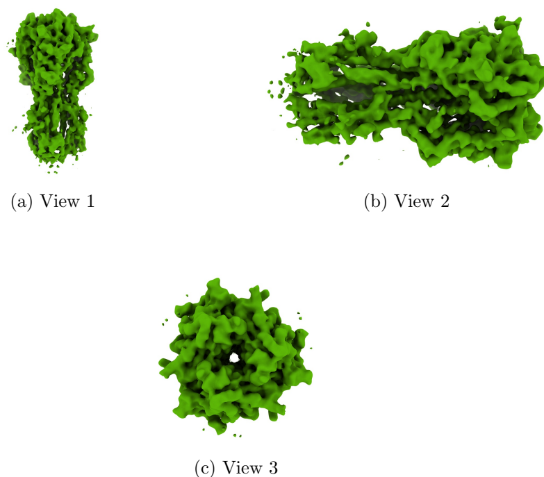
Figure 4: Isosurface at threshold=0.311000. Views generated by ChimeraX at a the following X, Y, Z angles: View 1 (0, -90, -90), View 2 (-90, 0, -90), View 3 (0, 0, 0).
