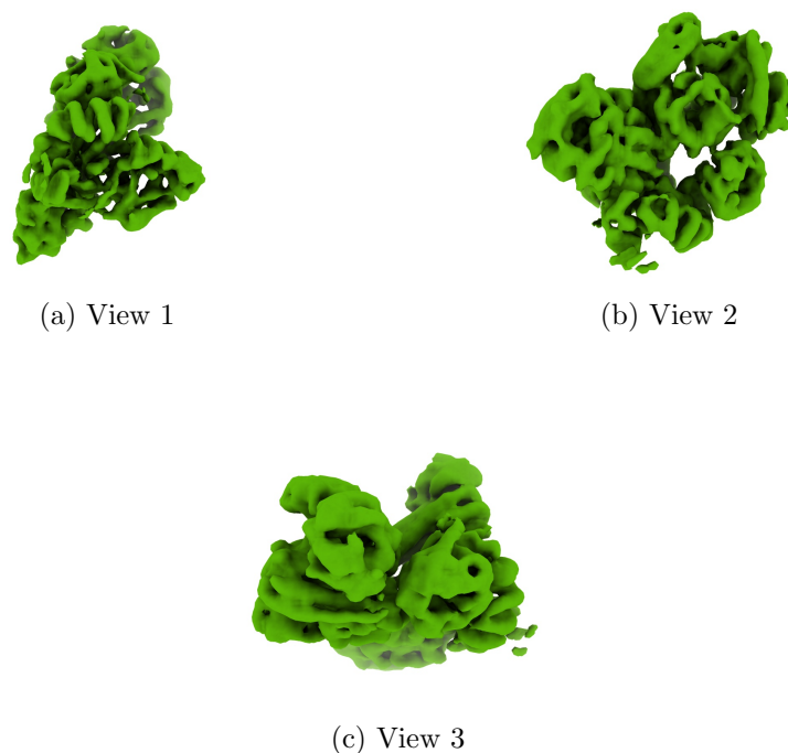
Figure 4: Isosurface at threshold=0.026500. Views generated by ChimeraX at a the following X, Y, Z angles: View 1 (0, -90, -90), View 2 (-90, 0, -90), View 3 (0, 0, 0).
