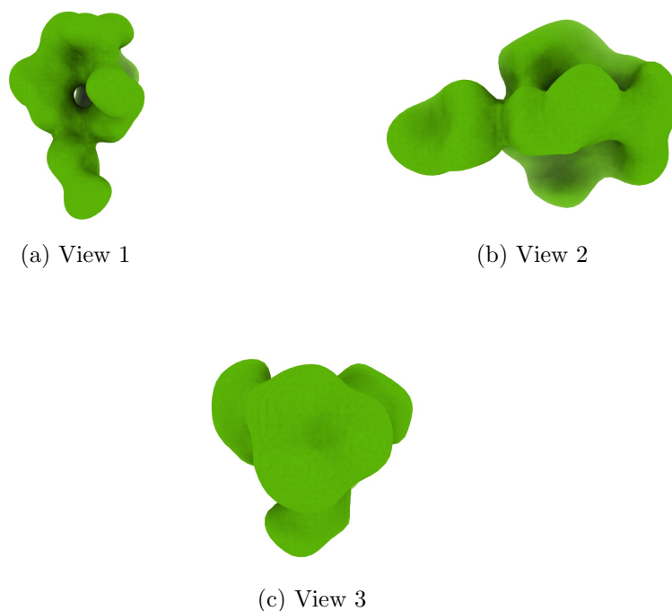
Figure 4: Isosurface at threshold=0.034400. Views generated by ChimeraX at a the following X, Y, Z angles: View 1 (0, -90, -90), View 2 (-90, 0, -90), View 3 (0, 0, 0).
