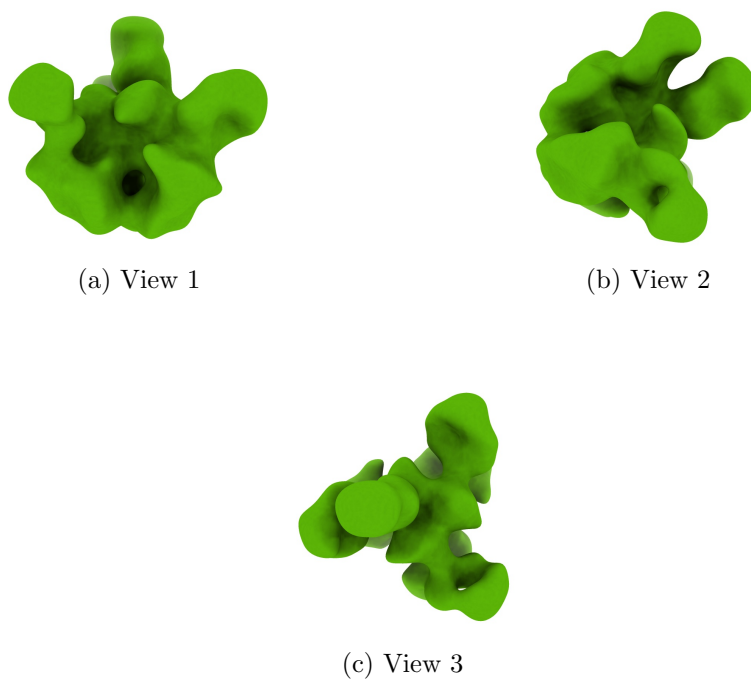
Figure 4: Isosurface at threshold=0.011800. Views generated by ChimeraX at a the following X, Y, Z angles: View 1 (0, -90, -90), View 2 (-90, 0, -90), View 3 (0, 0, 0).
