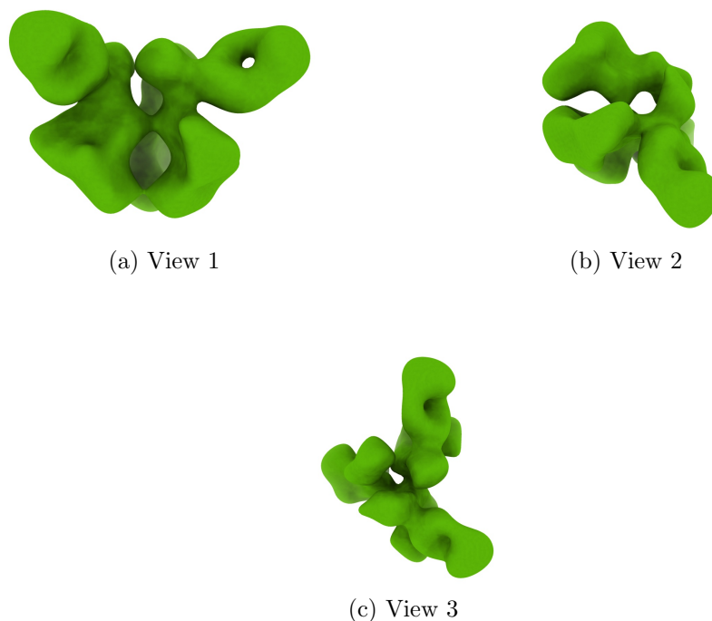
Figure 4: Isosurface at threshold=0.030200. Views generated by ChimeraX at a the following X, Y, Z angles: View 1 (0, -90, -90), View 2 (-90, 0, -90), View 3 (0, 0, 0).
