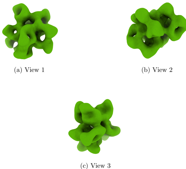
Figure 4: Isosurface at threshold=0.017900. Views generated by ChimeraX at a the following X, Y, Z angles: View 1 (0, -90, -90), View 2 (-90, 0, -90), View 3 (0, 0, 0).
