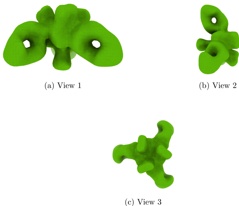
Figure 4: Isosurface at threshold=4.390000. Views generated by ChimeraX at a the following X, Y, Z angles: View 1 (0, -90, -90), View 2 (-90, 0, -90), View 3 (0, 0, 0).
