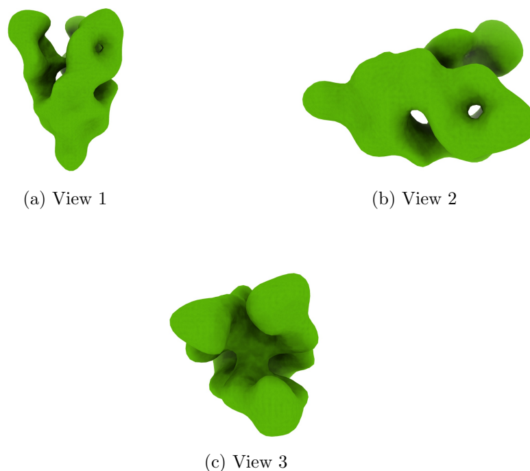
Figure 4: Isosurface at threshold=12.900000. Views generated by ChimeraX at a the following X, Y, Z angles: View 1 (0, -90, -90), View 2 (-90, 0, -90), View 3 (0, 0, 0).
