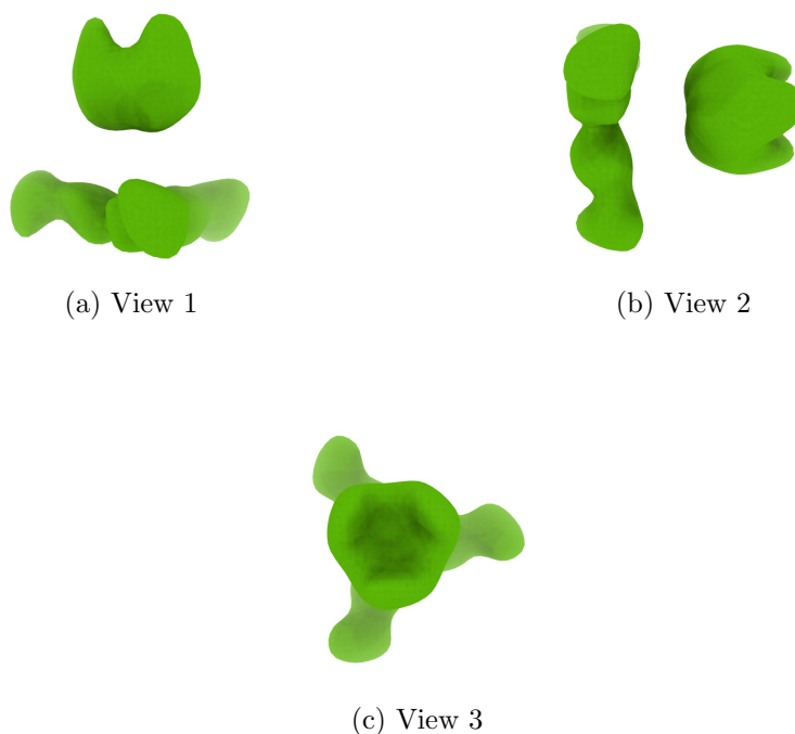
Figure 4: Isosurface at threshold=27.100000. Views generated by ChimeraX at a the following X, Y, Z angles: View 1 (0, -90, -90), View 2 (-90, 0, -90), View 3 (0, 0, 0).
