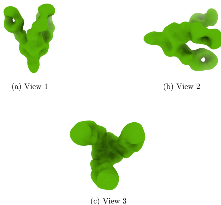
Figure 4: Isosurface at threshold=30.500000. Views generated by ChimeraX at a the following X, Y, Z angles: View 1 (0, -90, -90), View 2 (-90, 0, -90), View 3 (0, 0, 0).
