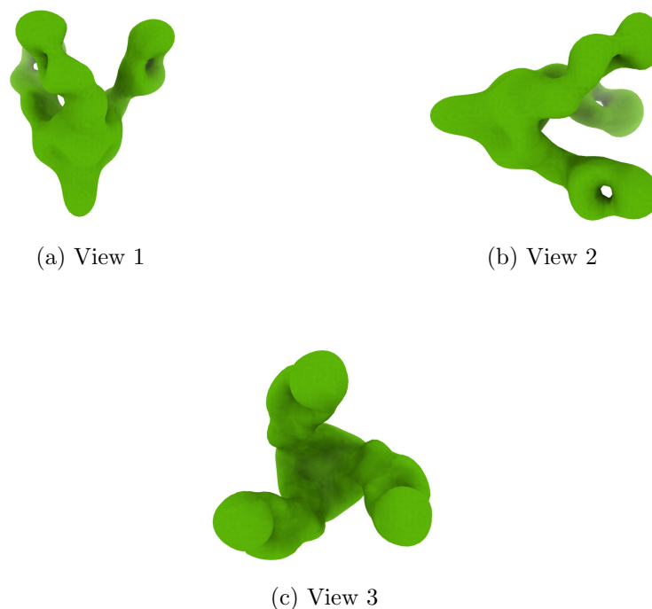
Figure 4: Isosurface at threshold=47.200000. Views generated by ChimeraX at a the following X, Y, Z angles: View 1 (0, -90, -90), View 2 (-90, 0, -90), View 3 (0, 0, 0).
