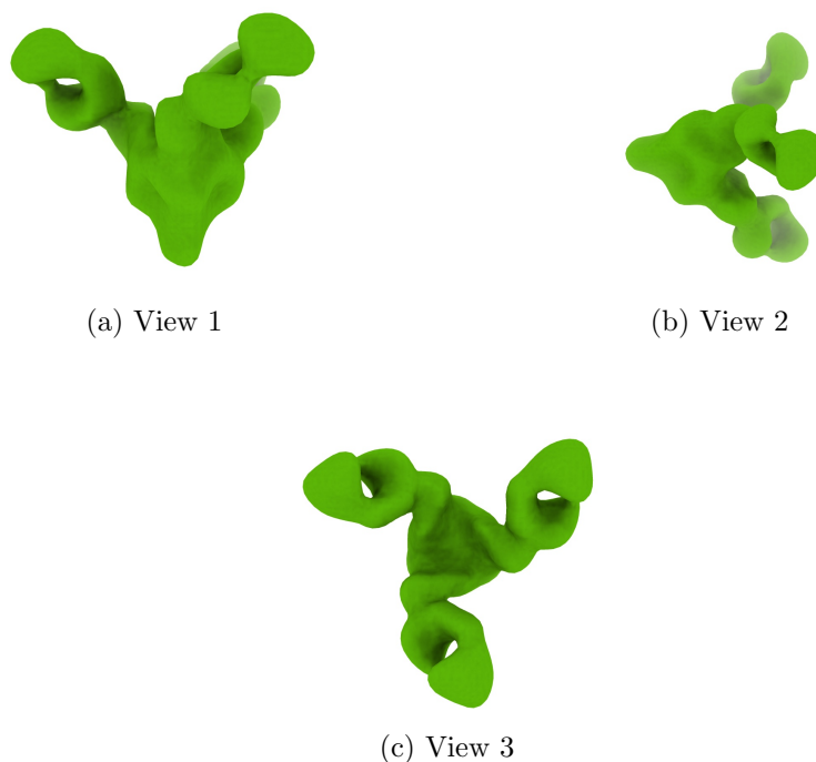
Figure 4: Isosurface at threshold=21.800000. Views generated by ChimeraX at a the following X, Y, Z angles: View 1 (0, -90, -90), View 2 (-90, 0, -90), View 3 (0, 0, 0).
