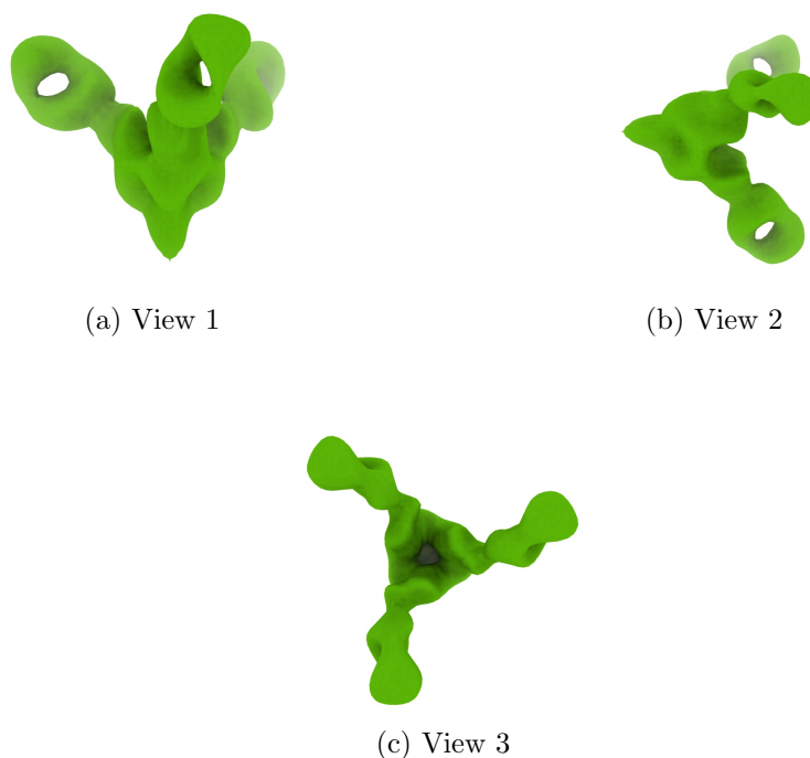
Figure 4: Isosurface at threshold=22.100000. Views generated by ChimeraX at a the following X, Y, Z angles: View 1 (0, -90, -90), View 2 (-90, 0, -90), View 3 (0, 0, 0).
