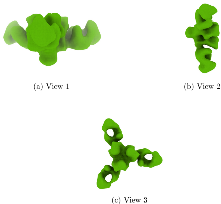
Figure 4: Isosurface at threshold=4.100000. Views generated by ChimeraX at a the following X, Y, Z angles: View 1 (0, -90, -90), View 2 (-90, 0, -90), View 3 (0, 0, 0).
