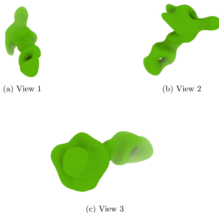
Figure 4: Isosurface at threshold=0.058500. Views generated by ChimeraX at a the following X, Y, Z angles: View 1 (0, -90, -90), View 2 (-90, 0, -90), View 3 (0, 0, 0).
