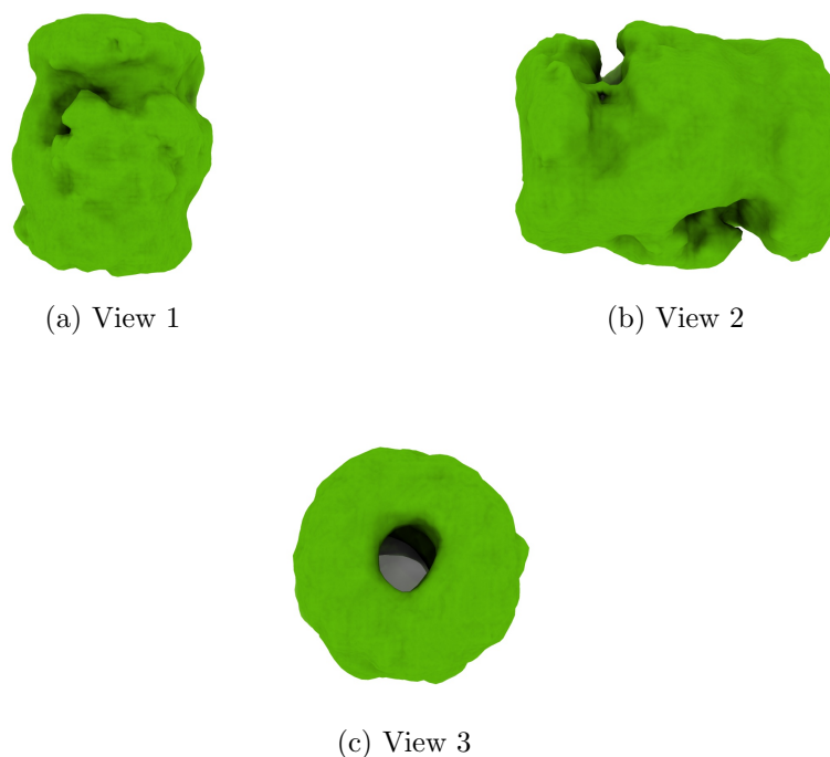
Figure 4: Isosurface at threshold=3.210000. Views generated by ChimeraX at a the following X, Y, Z angles: View 1 (0, -90, -90), View 2 (-90, 0, -90), View 3 (0, 0, 0).
