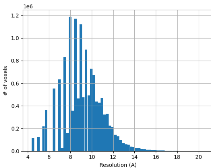
Figure 29: Histogram of the local resolution according to MonoRes.
