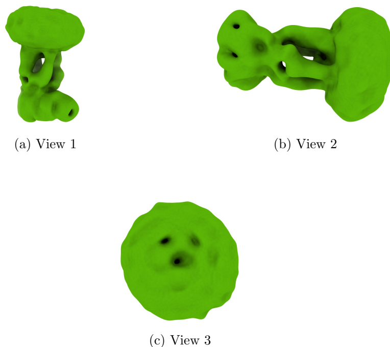
Figure 4: Isosurface at threshold=1.550000. Views generated by ChimeraX at a the following X, Y, Z angles: View 1 (0, -90, -90), View 2 (-90, 0, -90), View 3 (0, 0, 0).
