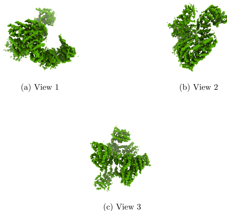
Figure 4: Isosurface at threshold=0.032400. Views generated by ChimeraX at a the following X, Y, Z angles: View 1 (0, -90, -90), View 2 (-90, 0, -90), View 3 (0, 0, 0).
