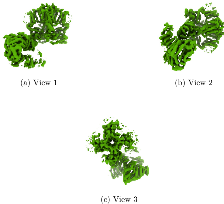
Figure 4: Isosurface at threshold=0.011100. Views generated by ChimeraX at a the following X, Y, Z angles: View 1 (0, -90, -90), View 2 (-90, 0, -90), View 3 (0, 0, 0).
