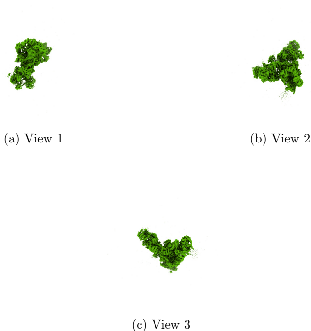
Figure 4: Isosurface at threshold=0.032000. Views generated by ChimeraX at a the following X, Y, Z angles: View 1 (0, -90, -90), View 2 (-90, 0, -90), View 3 (0, 0, 0).
