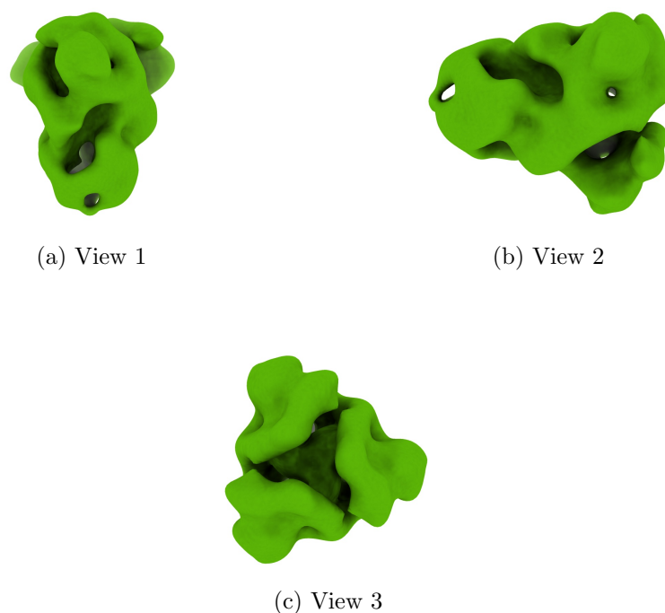
Figure 4: Isosurface at threshold=5.620000. Views generated by ChimeraX at a the following X, Y, Z angles: View 1 (0, -90, -90), View 2 (-90, 0, -90), View 3 (0, 0, 0).
