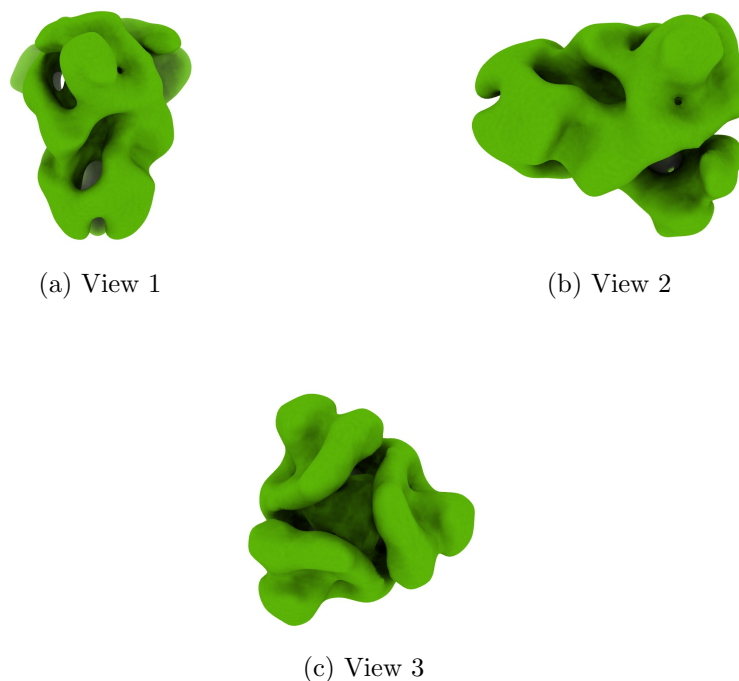
Figure 4: Isosurface at threshold=4.790000. Views generated by ChimeraX at a the following X, Y, Z angles: View 1 (0, -90, -90), View 2 (-90, 0, -90), View 3 (0, 0, 0).
