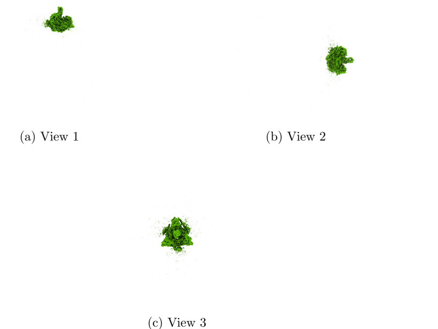
Figure 4: Isosurface at threshold=0.250000. Views generated by ChimeraX at a the following X, Y, Z angles: View 1 (0, -90, -90), View 2 (-90, 0, -90), View 3 (0, 0, 0).
