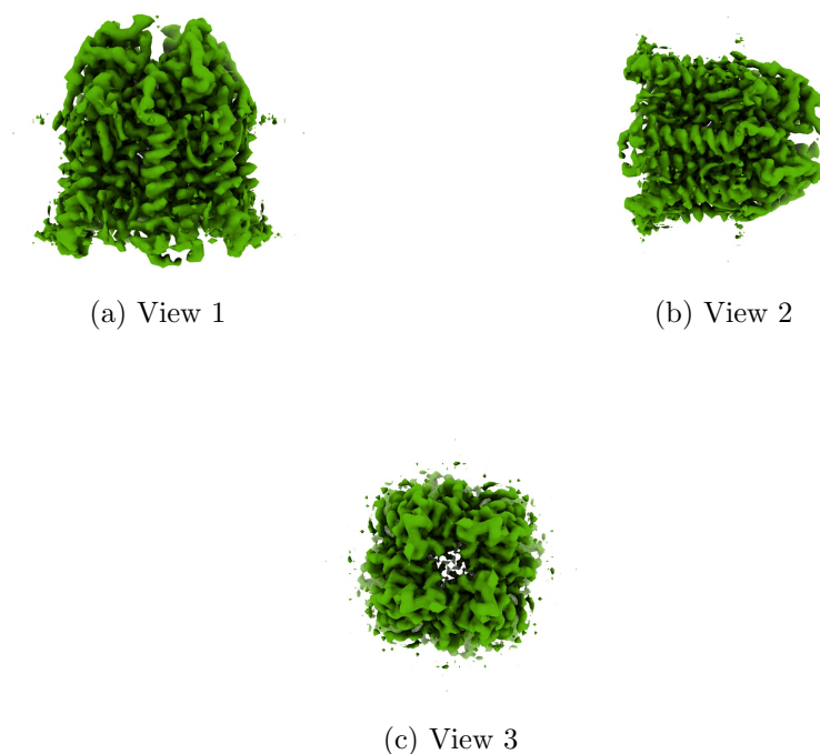
Figure 4: Isosurface at threshold=0.076700. Views generated by ChimeraX at a the following X, Y, Z angles: View 1 (0, -90, -90), View 2 (-90, 0, -90), View 3 (0, 0, 0).
