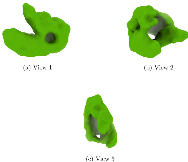
Figure 4: Isosurface at threshold=0.178000. Views generated by ChimeraX at a the following X, Y, Z angles: View 1 (0, -90, -90), View 2 (-90, 0, -90), View 3 (0, 0, 0).
