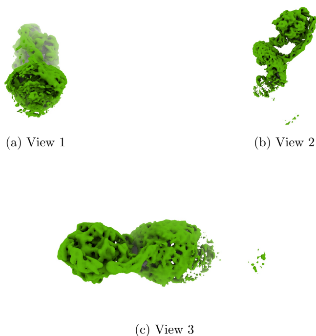
Figure 4: Isosurface at threshold=0.028000. Views generated by ChimeraX at a the following X, Y, Z angles: View 1 (0, -90, -90), View 2 (-90, 0, -90), View 3 (0, 0, 0).
