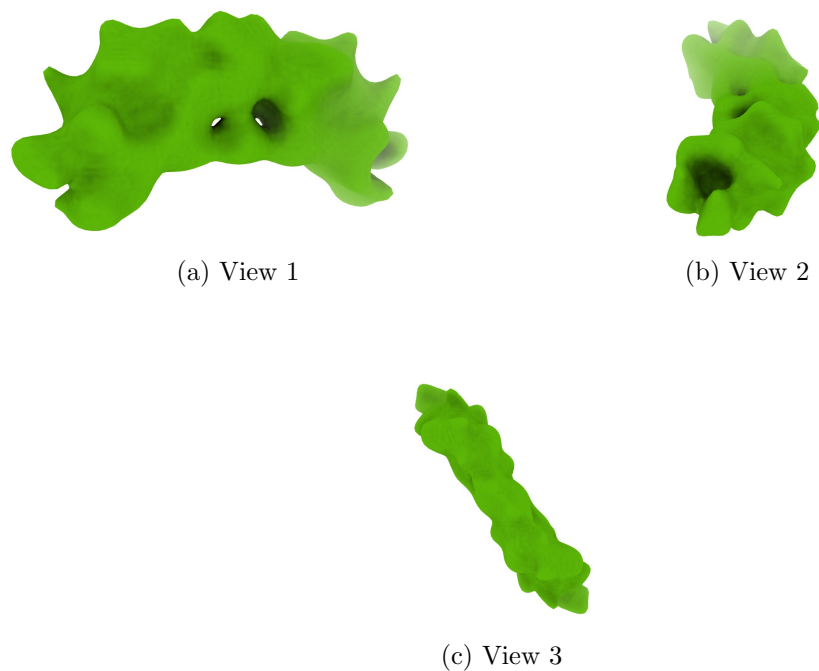
Figure 4: Isosurface at threshold=0.123000. Views generated by ChimeraX at a the following X, Y, Z angles: View 1 (0, -90, -90), View 2 (-90, 0, -90), View 3 (0, 0, 0).
