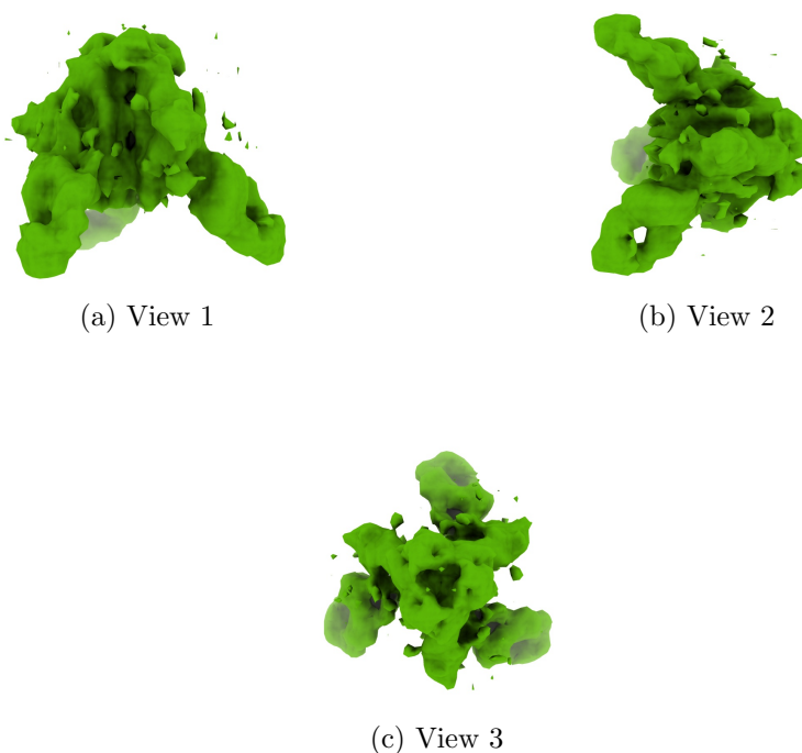
Figure 4: Isosurface at threshold=1.560000. Views generated by ChimeraX at a the following X, Y, Z angles: View 1 (0, -90, -90), View 2 (-90, 0, -90), View 3 (0, 0, 0).
