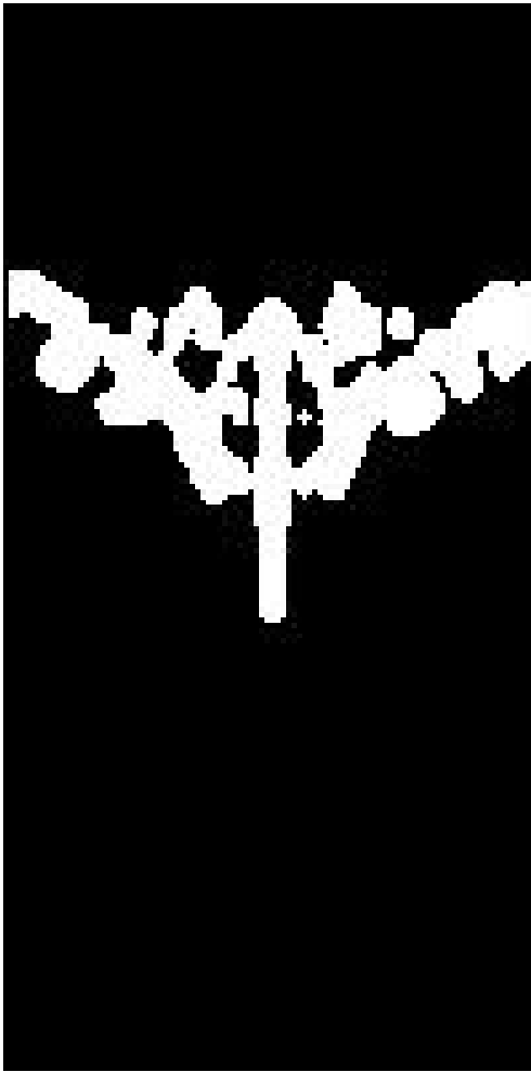
(a) X Slice 50
