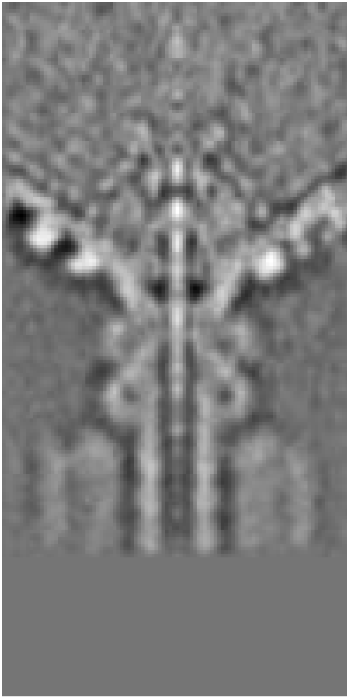
(a) X Slice 50
