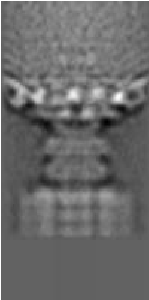
(a) X Projection
