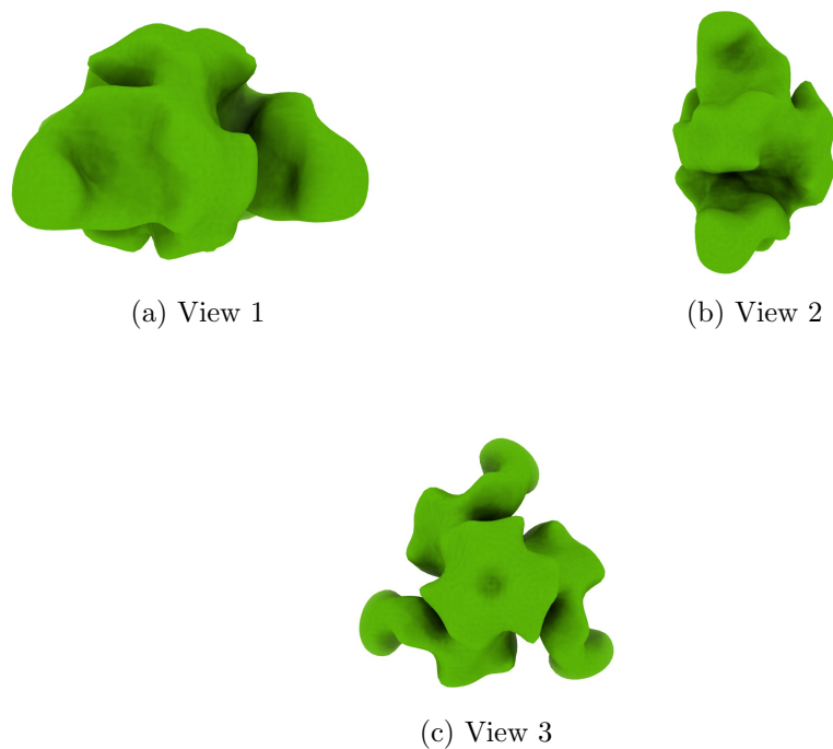
Figure 4: Isosurface at threshold=21.100000. Views generated by ChimeraX at a the following X, Y, Z angles: View 1 (0, -90, -90), View 2 (-90, 0, -90), View 3 (0, 0, 0).
