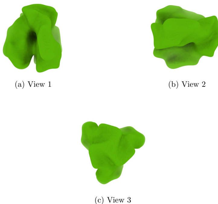
Figure 4: Isosurface at threshold=13.500000. Views generated by ChimeraX at a the following X, Y, Z angles: View 1 (0, -90, -90), View 2 (-90, 0, -90), View 3 (0, 0, 0).
