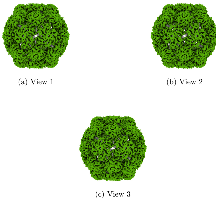
Figure 4: Isosurface at threshold=0.039200. Views generated by ChimeraX at a the following X, Y, Z angles: View 1 (0, -90, -90), View 2 (-90, 0, -90), View 3 (0, 0, 0).
