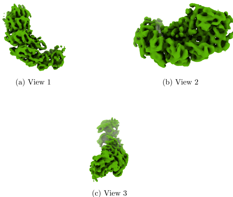
Figure 4: Isosurface at threshold=0.082000. Views generated by ChimeraX at a the following X, Y, Z angles: View 1 (0, -90, -90), View 2 (-90, 0, -90), View 3 (0, 0, 0).
