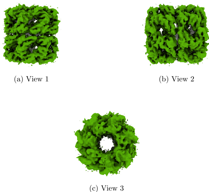
Figure 4: Isosurface at threshold=0.090000. Views generated by ChimeraX at the following X, Y, Z angles: View 1 (0, -90, -90), View 2 (-90, 0, -90), View 3 (0, 0, 0).
